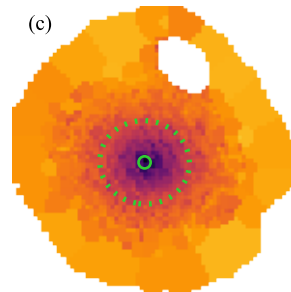
\log \Sigma_{\star}^{\text{dez}} [M_{\odot} \text{ pc}^{-2}]
