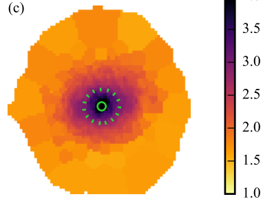
\log \Sigma_{\star}^{\text{dez}} [\text{M}_{\odot} \text{pc}^{-2}]
