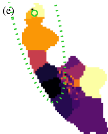
\langle \log Z \rangle_M [ Z_{\odot} ]
