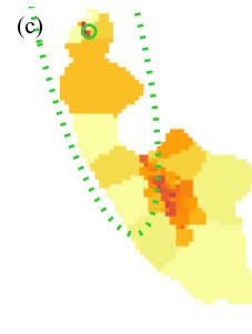
\log \Sigma_{\star}^{\text{dez}} [ M_{\odot} \text{pc}^{-2} ]
