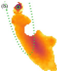
\log \mathcal{L}_{5635\text{\AA}} [ L_{\odot} \text{pc}^{-2} ]
