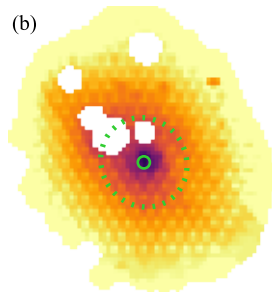
\log \mathcal{L}_{5635\text{\AA}} [L_{\odot} \text{pc}^{-2}]
