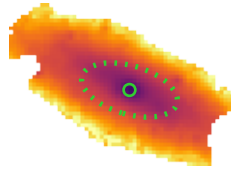
\langle \log Z \rangle_M [Z_{\odot}]
