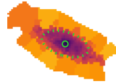
\log \Sigma_{\star}^{\text{dez}} [M_{\odot} \text{pc}^{-2}]
