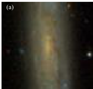
SDSS image
