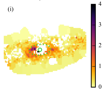
\sigma_{\star} [\text{kms}^{-1}]
