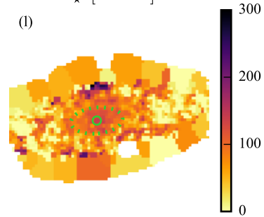
\sigma_{\star} [\text{kms}^{-1}]
