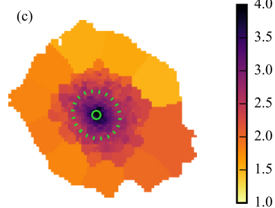
\log \Sigma_{\star}^{\text{dex}} [ M_{\odot} \text{pc}^{-2} ]
