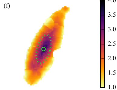
b^{\text{gal}}
