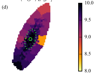
\log \Sigma_{\text{SFR}} [M_{\odot} \text{Gyr}^{-1} \text{pc}^{-2}]
