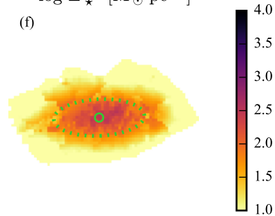
b^{\text{gal}}
