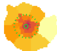
\log \Sigma_{\star}^{\text{dez}} [ M_{\odot} \text{pc}^{-2} ]
