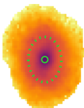
\langle \log Z \rangle_M [Z_{\odot}]
