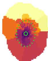
\log \Sigma_{\star}^{\text{dez}} [\text{M}_{\odot} \text{pc}^{-2}]
