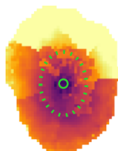
b^{\text{gal}}
