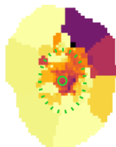
\sigma_{\star} [\text{km s}^{-1}]
