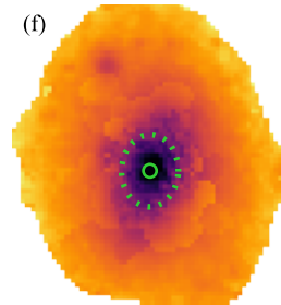
\log \Sigma_{\star}^{\text{dez}} [M_{\odot} \text{pc}^{-2}]
