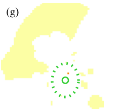
\log \Sigma_{\text{SFR}} [M_{\odot} \text{Gyr}^{-1} \text{pc}^{-2}]
