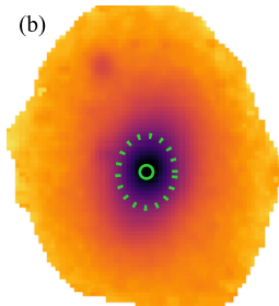
\log \mathcal{L}_{5635\text{\AA}} [L_{\odot} \text{pc}^{-2}]
