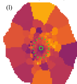
\sigma_{\star} [\text{km s}^{-1}]
