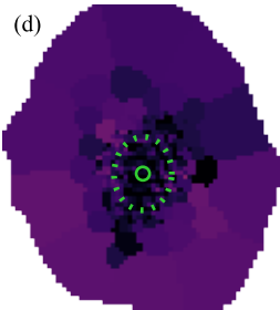
\langle \log t \rangle_L [\text{yr}]
