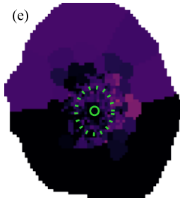
\langle \log Z \rangle_M [Z_{\odot}]
