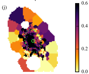
\tau_V
