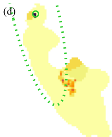
\langle \log t \rangle_L [yr]
