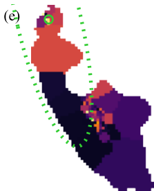
\langle \log Z \rangle_M [ Z_{\odot} ]
