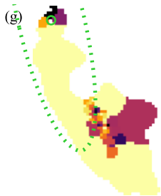
\log \Sigma_{\text{SFR}} [ M_{\odot} \text{Gyr}^{-1} \text{pc}^{-2} ]
