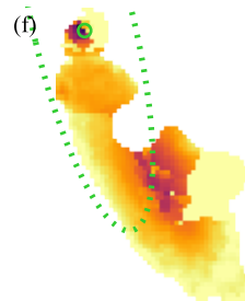
\log \Sigma_{\star}^{\text{dez}} [ M_{\odot} \text{pc}^{-2} ]
