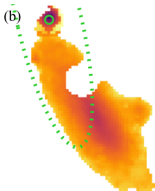
\log \mathcal{L}_{5635\text{\AA}} [ L_{\odot} \text{pc}^{-2} ]
