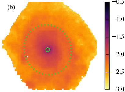
\langle \log Z \rangle_{\text{M}} [Z_{\odot}]
