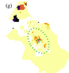
\log \Sigma_{\text{SFR}} [ M_{\odot} \text{Gyr}^{-1} \text{pc}^{-2} ]
