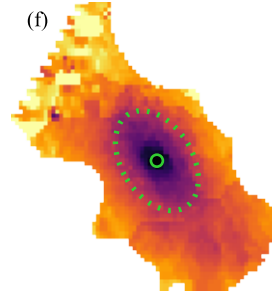
\log \Sigma_{\star}^{\text{dez}} [ M_{\odot} \text{pc}^{-2} ]
