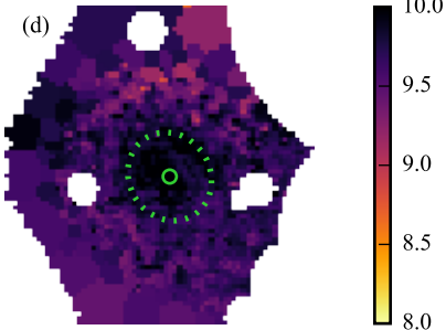
\log \Sigma_{\text{SFR}} [M_{\odot} \text{Gyr}^{-1} \text{pc}^{-2}]
