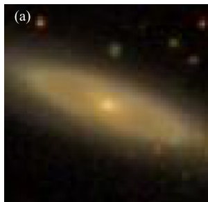
\langle \log t \rangle_L [\text{yr}]
