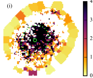
b^{\text{gal}}
