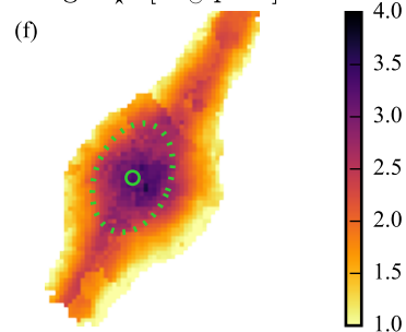
b^{\text{gal}}
