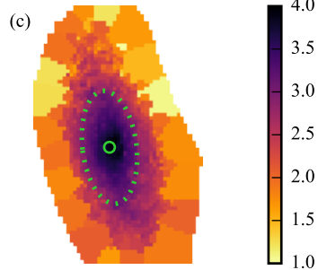
\log \Sigma_{\star}^{\text{dez}} [\text{M}_{\odot} \text{pc}^{-2}]
