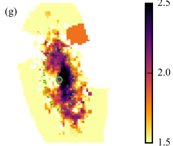
\log \Sigma_{\text{SFR}} [\text{M}_{\odot} \text{Gyr}^{-1} \text{pc}^{-2}]
