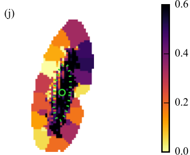
\tau_V
