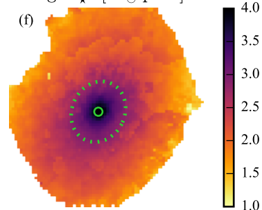
b^{\text{gal}}
