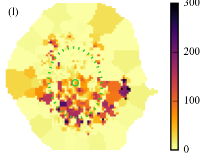
\sigma_{\star} [\text{kms}^{-1}]
