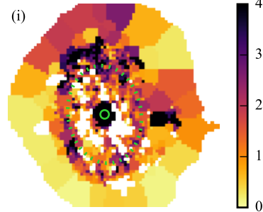
\sigma_{\star} [\text{kms}^{-1}]
