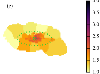
\log \Sigma_{\star}^{\text{dez}} [M_{\odot} \text{pc}^{-2}]
