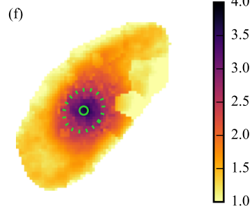
b^{\text{gal}}
