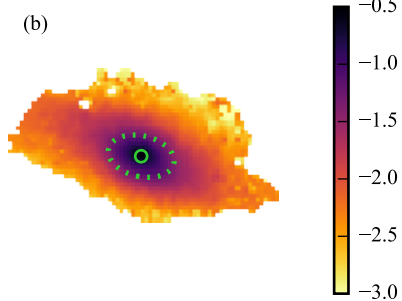
\langle \log Z \rangle_{\text{M}} [Z_{\odot}]
