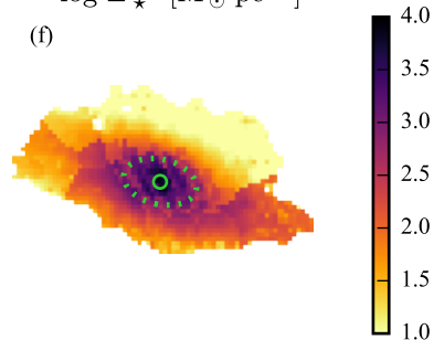
b^{\text{gal}}
