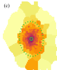
\log \Sigma_{\star}^{\text{dez}} [M_{\odot} \text{pc}^{-2}]
