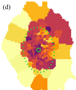
\langle \log t \rangle_L [\text{yr}]
