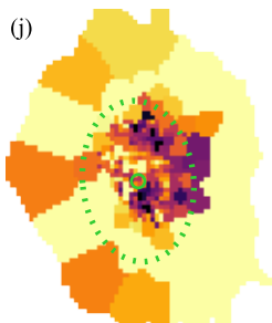
\tau_V
