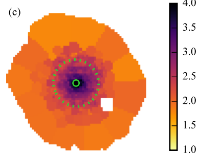
\log \Sigma_{\star}^{\text{dez}} [\text{M}_{\odot} \text{pc}^{-2}]
