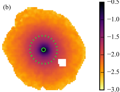
\langle \log Z \rangle_M [Z_{\odot}]
