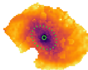
b^{\text{gal}}
