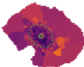
\log \Sigma_{\text{SFR}} [ M_{\odot} \text{Gyr}^{-1} \text{pc}^{-2} ]
