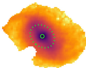
\langle \log Z \rangle_M [ Z_{\odot} ]
