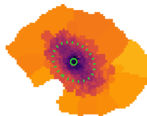
\log \Sigma_{\star}^{\text{dez}} [ M_{\odot} \text{pc}^{-2} ]
