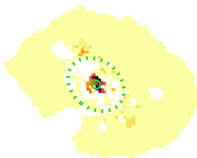
\tau_V
