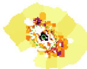
\sigma_{\star} [ \text{km s}^{-1} ]
