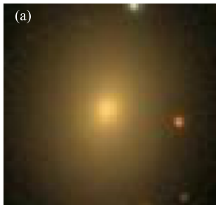
SDSS image
