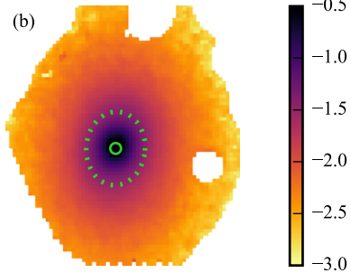
\langle \log Z \rangle_{\text{M}} [Z_{\odot}]
