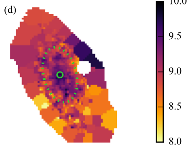
\log \Sigma_{\text{SFR}} [\text{M}_{\odot} \text{Gyr}^{-1} \text{pc}^{-2}]
