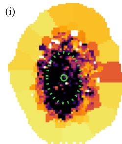
\sigma_{\star} [\text{km s}^{-1}]
