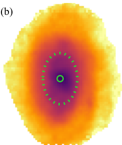
\log \mathcal{L}_{5635\text{\AA}} [\text{L}_{\odot} \text{pc}^{-2}]
