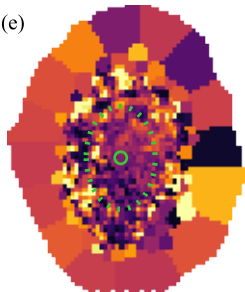
\langle \log Z \rangle_{\text{M}} [Z_{\odot}]
