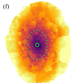
\log \Sigma_{\star}^{\text{dez}} [\text{M}_{\odot} \text{pc}^{-2}]
