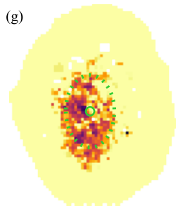
\log \Sigma_{\text{SFR}} [\text{M}_{\odot} \text{Gyr}^{-1} \text{pc}^{-2}]
