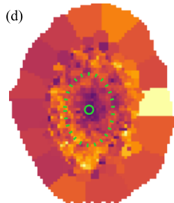
\langle \log t \rangle_{\text{L}} [\text{yr}]
