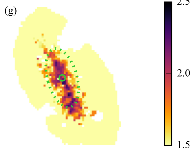
\log \Sigma_{\text{SFR}} [\text{M}_{\odot} \text{Gyr}^{-1} \text{pc}^{-2}]
