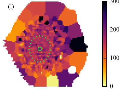
\sigma_{\star} [\text{kms}^{-1}]
